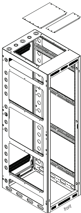
The rack includes a rear door and top closure panels (rear door can be omitted if not needed, see ordering option, pg. 2). A front door is optional, order separately.
