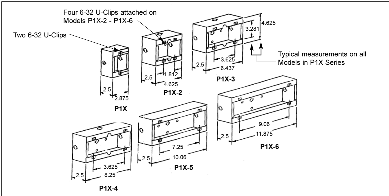
P1X Series Dimensions
