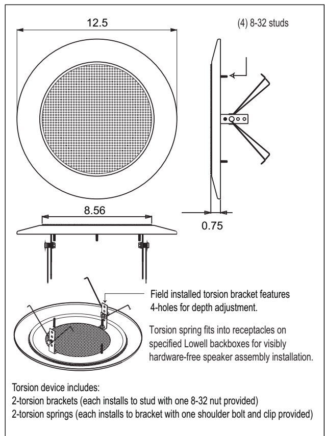
CN-8M Steel grille with torsion mount for visibly hardware-free appearance
