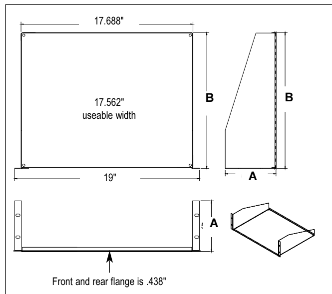
L15 Series Dimensions
